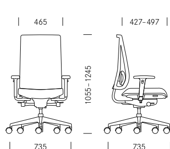
Swivel chair, backrest standard Bureaustoel, rug standaard
