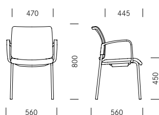
Four-legged chair | Cantilever chair Vierpoots stoel | Sledestoel
