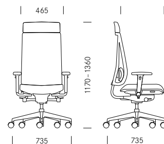
Swivel chair, with backrest extension Bureaustoel, met rugverlenging
